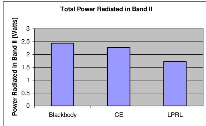
Figure 4: Total power radiated in band II for blackbody, and blackbody coated with indicated coatings. In band II, the blackbody radiates 2.44 W, the CE coated blackbody radiates 2.27 W, and the LPRL coated blackbody radiates 1.72 W.
