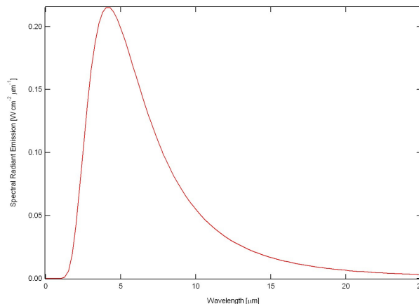
Figure 1: The Spectral Radiant Emission of a blackbody at 700 K.
