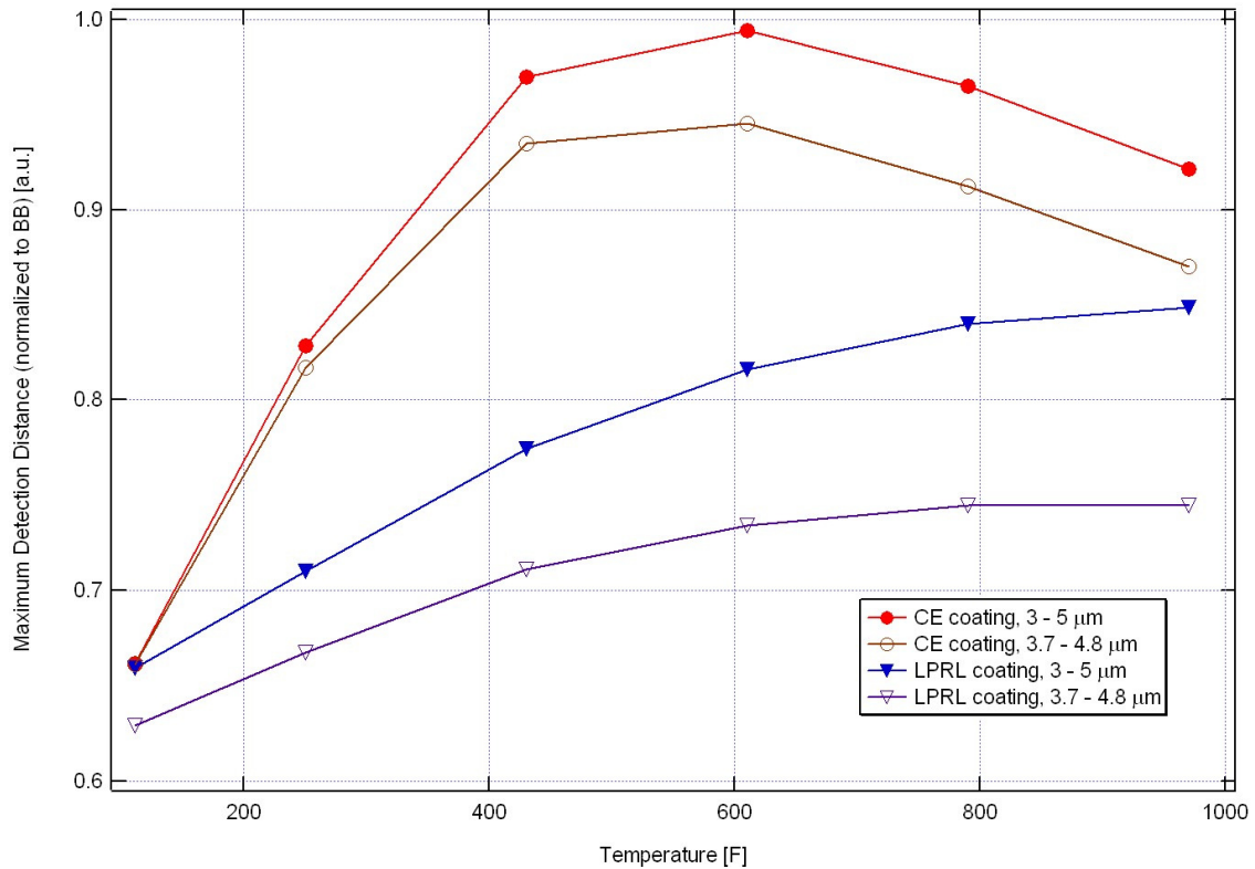
Figure 5: The maximum detection distance for the heated cubic centimeter black body coated with the LPRL coating (blue curve) and the constant emissivity (CE) coating (red curve). Both curves are normalized to the maximum detection distance of the black body cube (see Equation 7). For each coating, we show the result for band II (3 to 5 μm), and for the portion of the band detected by most IR detectors (3.7 to 4.8 μm).
